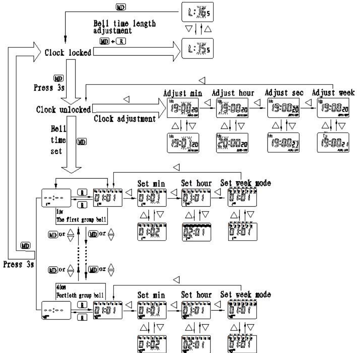
Figure6 TM624 TIME SWITCH of Belling apparatus Setting process
