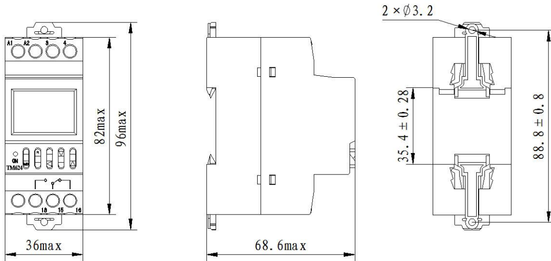
a) TM624 outside dimension
