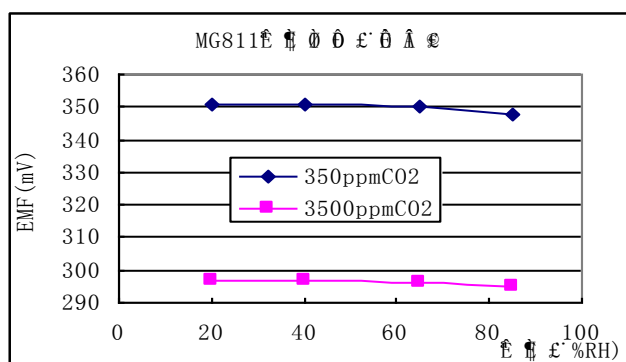
Fig6. Typical humidity characteristics
